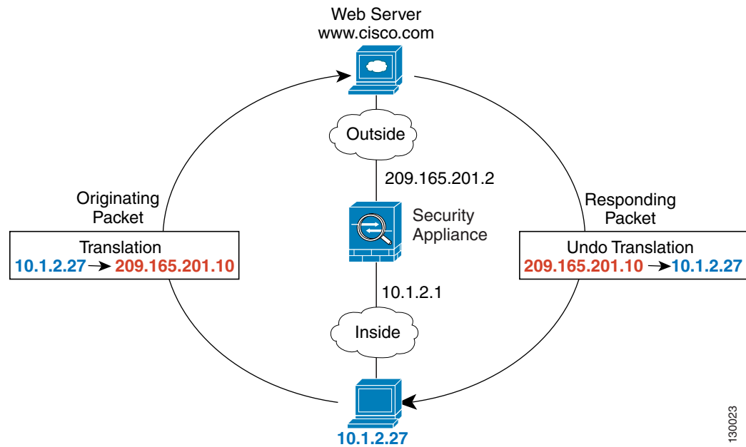
Figure 14-1 NAT Example
