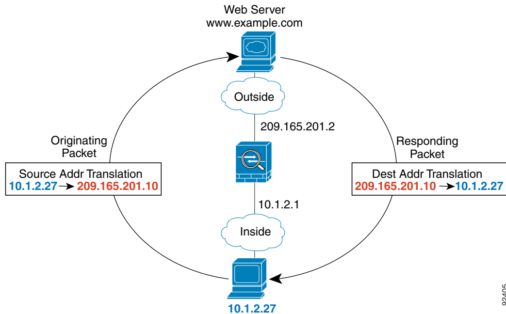
Figure 12-1 NAT Example
