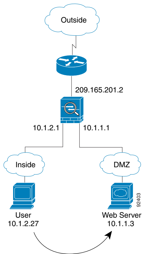
Figure 12-4 Inside to DMZ
