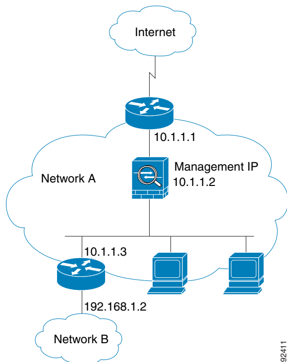
Figure 12-7 Transparent Firewall Network
